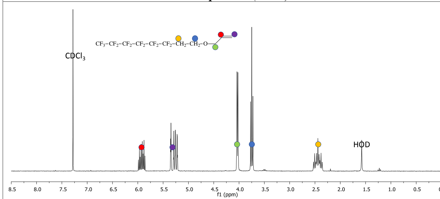
1 H NMR Spectrum (CDCl 3 )
