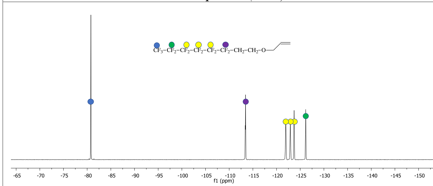
19 F NMR Spectrum (CDCl 3 )
