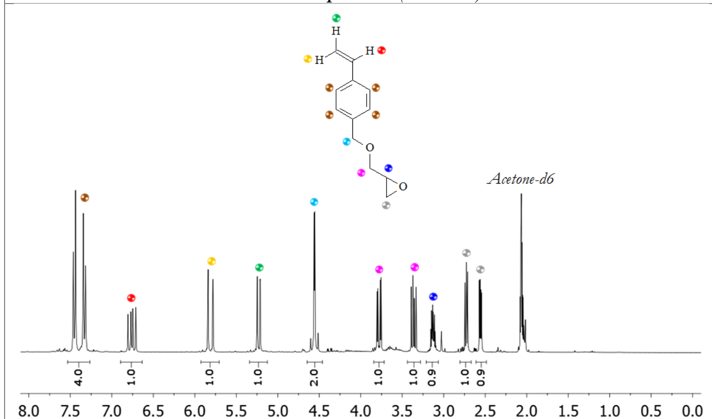
^1\text{H} NMR Spectrum ( Acetone-d6 )
