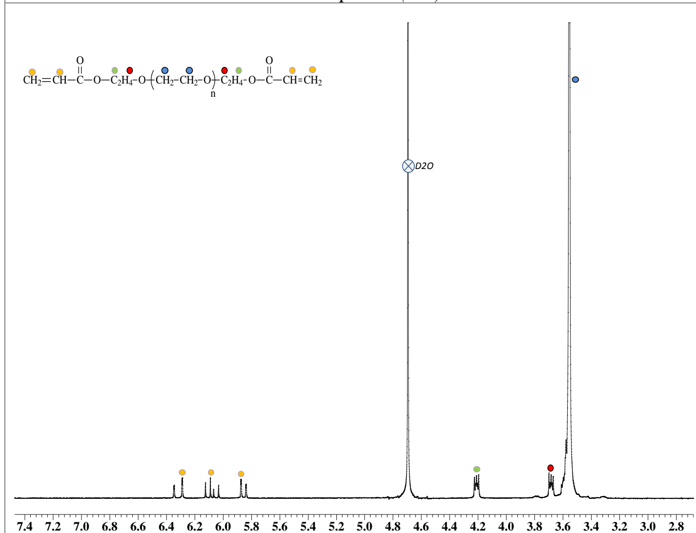
^1\text{H} NMR Spectrum ( D_2O )
