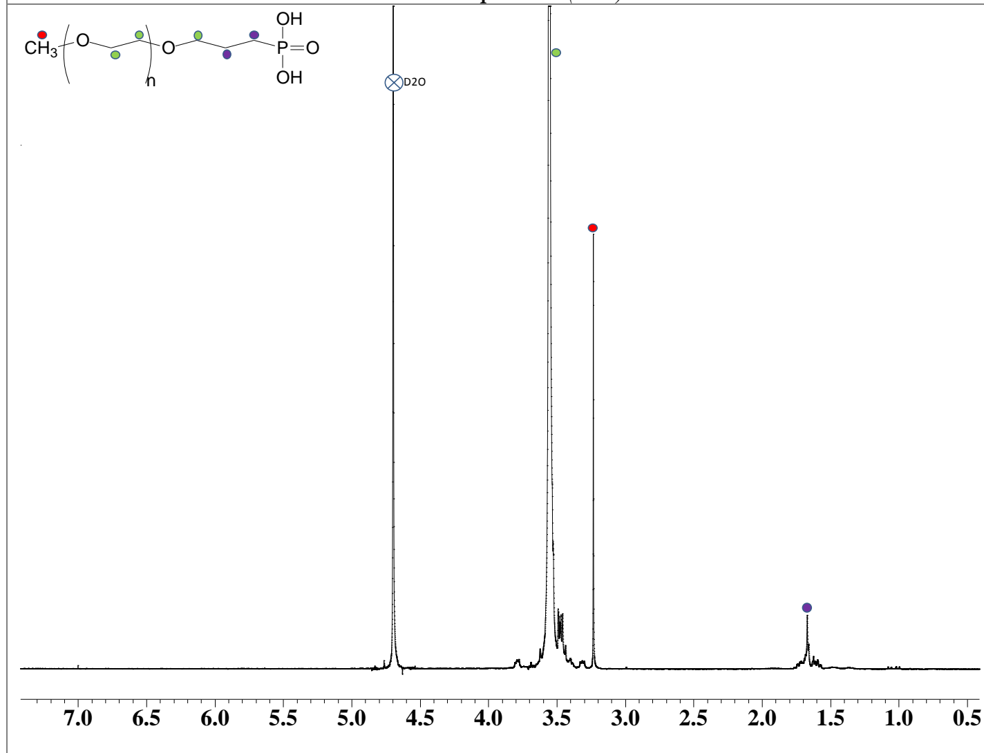
^1\text{H} NMR Spectrum ( \text{D}_2\text{O} )
