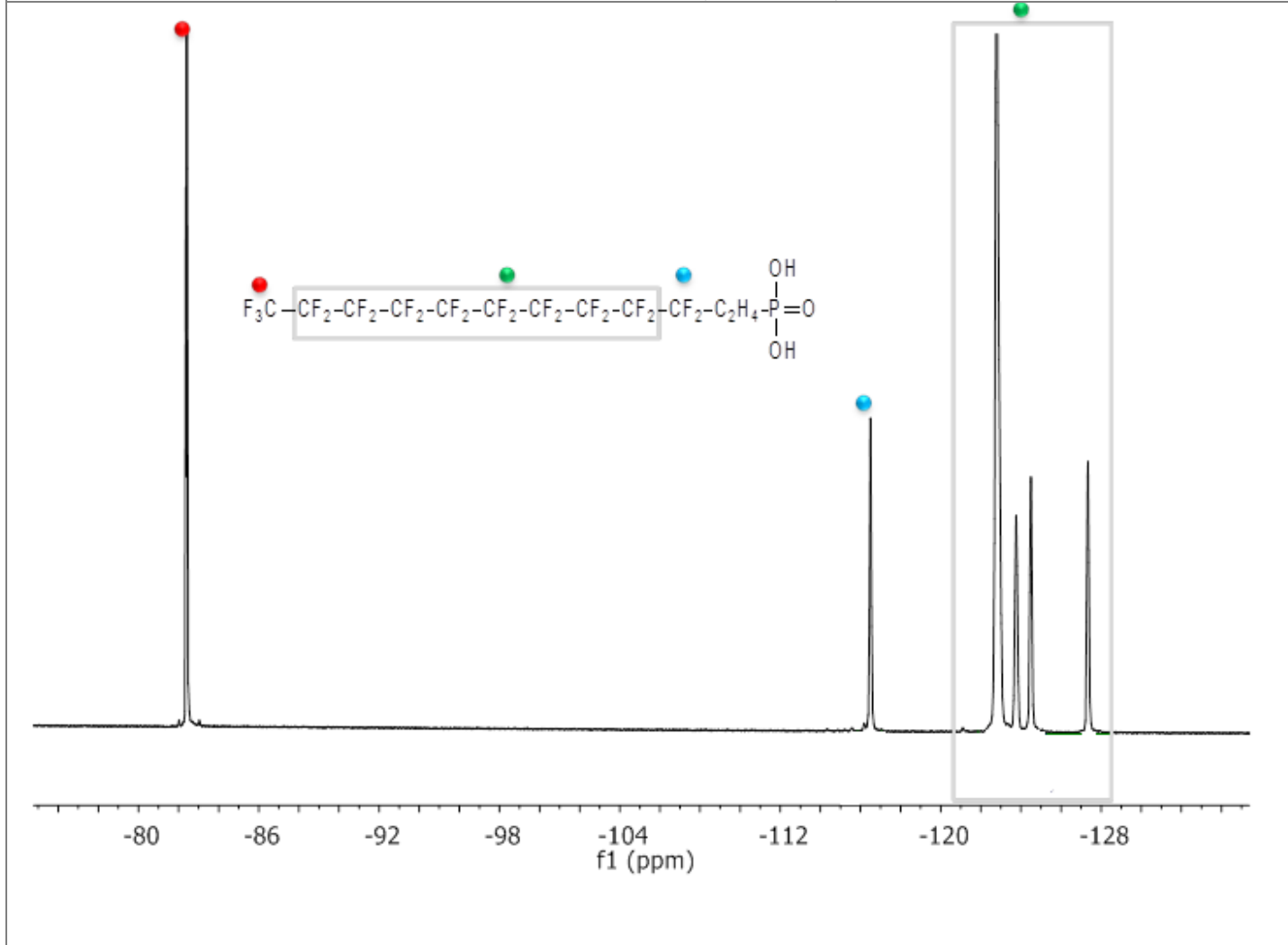
^{19}\text{F} NMR Spectrum (Methanol- d_4 )
