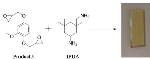
Scheme 6 Material prepared from Product 5 and IPDA.
